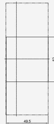
◆ PANEL CUT
