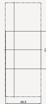
◆ PANEL CUT
