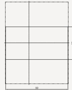
◆ PANEL CUT
